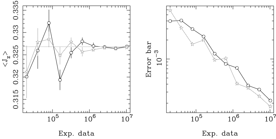
Fig. 1. Monte Carlo comparison between continuous and discrete tomography for a spin s = 1/2 system. Continuous tomography uses \hat{D}(\psi, \vec{n}) as quorum, while discrete tomography uses the quorum \mathcal{Q} \stackrel{\text{def}}{=} \{\hat{\sigma}_x, \hat{\sigma}_y, \hat{\sigma}_z, \hat{1}\} . Left: convergence of the mean value of \langle s_z \rangle for a coherent \alpha = 2 spin state for increasing number of experimental data (the theoretical value is given by the horizontal line). The circles \circ refer to continuous, the stars \star to discrete tomography. Right: plot of the statistical error bars of the graphs on the left vs experimental data. The error bars are obtained by dividing the experimental data into 20 statistical blocks. Notice that the two tomographic procedures are essentially equivalent.
