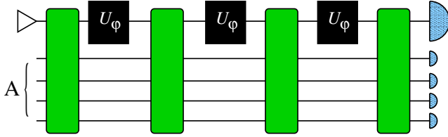
FIG. 2 (color online). Sequential (or multiround) protocol with a single probe. Thanks to the ancillary systems A , this scheme encompasses also adaptive techniques where information on \varphi is extracted between successive applications of the unitary U_\varphi . As in Fig. 1, the triangle represents the probe state preparation, the black squares represent U_\varphi , the symbols on the right represent detection, and the gray boxes represent unitary operations involving both the probe and the ancillas.
