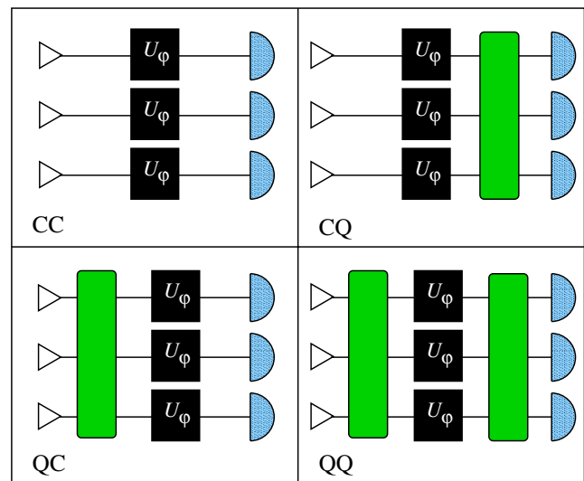
FIG. 1 (color online). Different strategies for the estimation of a parameter \varphi involving N parallel samplings of a unitary operator U_\varphi (black squares). The CC strategy involves separable input states and separable measurements [i.e., local operations and measurements whose results are communicated classically (LOCC)]. The CQ strategy involves separable input states and general measurement schemes. The QC strategy involves general input states (also entangled) and separable measurements. The QQ strategy involves general input states and general measurement schemes. The triangles on the left represent state preparation and the symbols on the right represent measurements. The gray boxes represent a unitary operation involving multiple probes (Q strategies).
