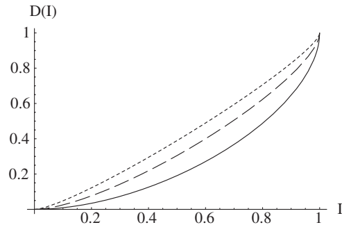
FIG. 1. Optimal information-disturbance tradeoff in estimating an unknown maximally entangled state for dimension d = 2 (solid line), d = 4 (dashed line), and d = 8 (dotted line), where I and D are defined through Eqs. (25) and (26) in terms of the estimation and operation fidelities G and F , respectively. For given value of the retrieved information I , the curves D(I) are a lower bound for the disturbance of any measurement instrument.
