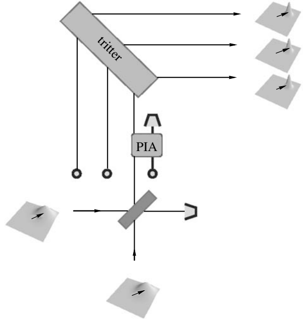
Experimental scheme to achieve optimal superbroadcasting from 2 to 3 copies. This setup involves just a beam splitter, a phase-insensitive amplifier and a tritter, which in turn can be implemented by two suitably balanced beam splitters. The phase-insensitive amplifier can be implemented by a beam splitter and heterodyne-assisted feed-forward. The output copies carrying the same signal as the input ones are locally more pure, the noise being shifted to classical correlations between them.
